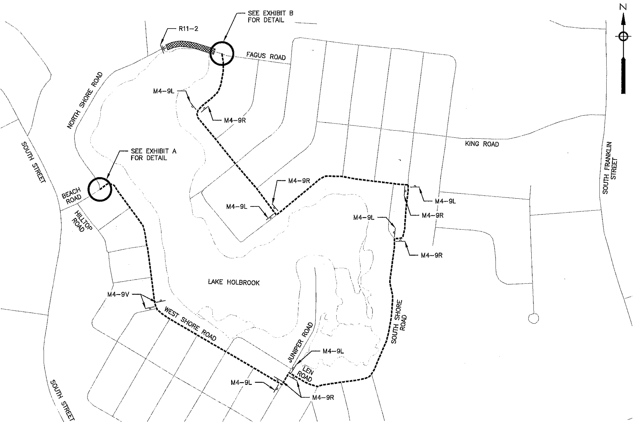
NORTH SHORE ROAD DETOUR PLAN
